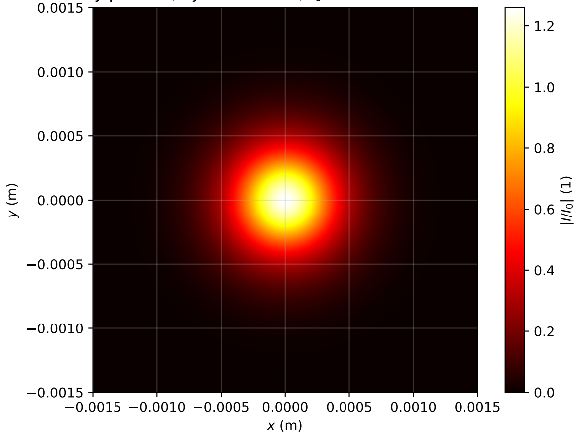
Intensity profile I(x, y, z = 0.716m)/I_0 , Pin=0.9Pcr, artificial time
